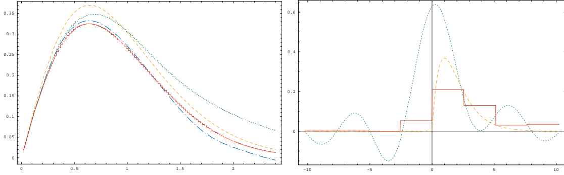
FIGURE 2. Left: Imaginary part of the empirical (dot-dashed blue), true (orange dashed), pilot (dotted green) and final estimated (red solid) characteristic function. Right: pilot (dotted green), final (red solid) estimator and true (dashed orange) density of \nu_\sigma ; the pilot estimator does not have a point mass in zero.
